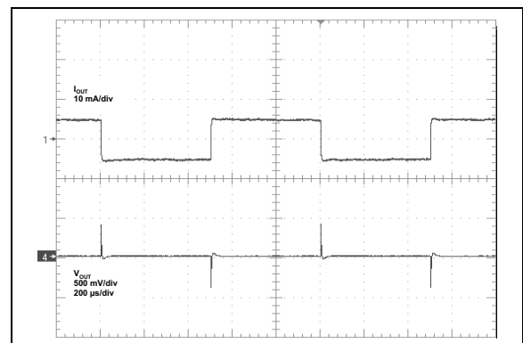
FIGURE 2-24: Load Transient, V_{DD} = 5.5 , V_{IN} = 2.5 , 2.048V Option.
