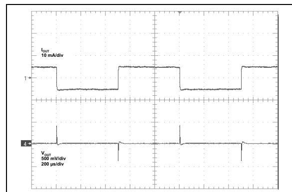
FIGURE 2-24: Load Transient, V_{DD} = 5.5\text{V} , V_{IN} = 2.5 , 2.048V Option.
