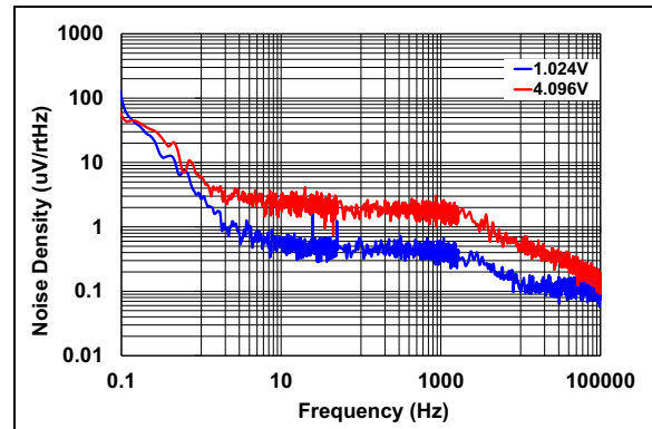
FIGURE 2-12: Noise vs. Frequency, No Load, T_A = +25^{\circ}C .
