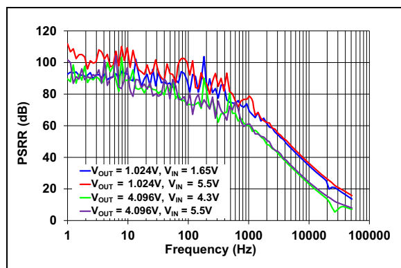
FIGURE 2-14: PSRR vs. Frequency, 1 kΩ Load, T_A = +25^\circ\text{C} .
