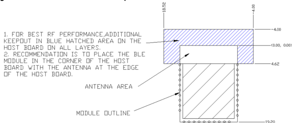
Figure 3. Recommended Host PCB Keep Out Area Around the CYBLE-212019-00 Antenna
