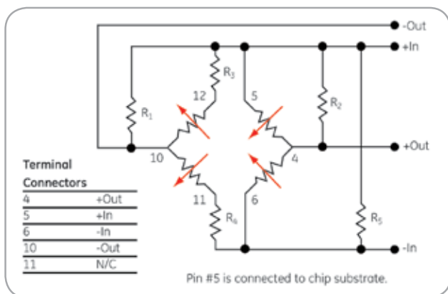
NPH Series schematic diagram
