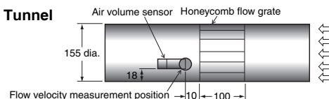
Figure 2: Wind Tunnel
