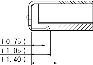
SEC A-A(S=10/1)
