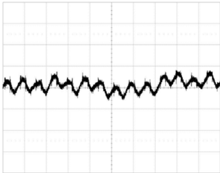
Output voltage ripple (5 mV/div.) at: T_{ref} = +25^{\circ}C , I_O = 60 A electrical load, V_I = 5 V . Time scale: 5 μs/div. Output capacitor: 660 μF electrolysis type. See the filter in the Output ripple and noise section (EMC Specification).
