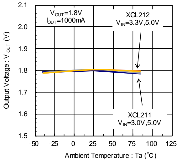
(4) Output Voltage vs. Ambient Temperature V_{OUT}=1.8V
