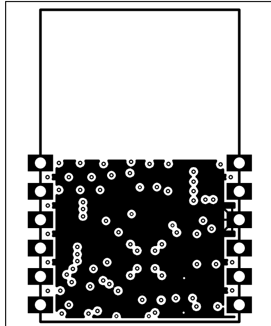
FIGURE 2-6: POWER PLANE
