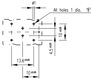
29 PCB plug-in base page 131
