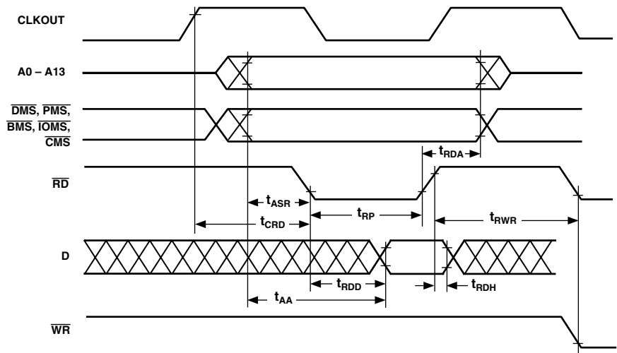
Figure 11. Memory Read
