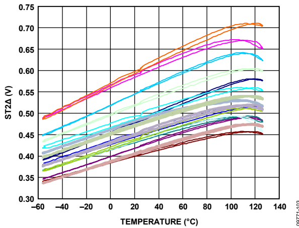
Figure 14. ST2 Output Change vs. Temperature, 16 Parts in Sockets
