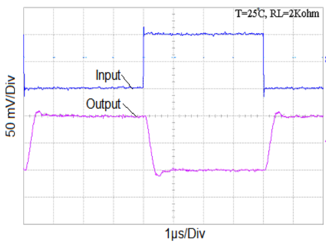
Inverting Small Signal Pulse Response
