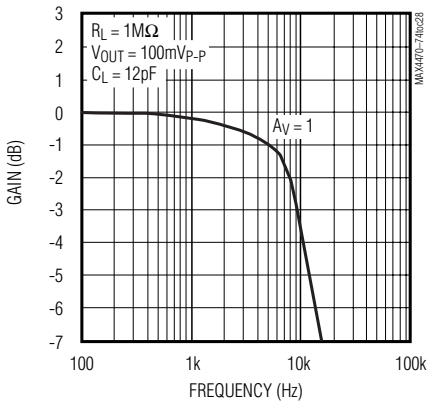
MAX4470/MAX4471/MAX4472 SMALL-SIGNAL GAIN vs. FREQUENCY
