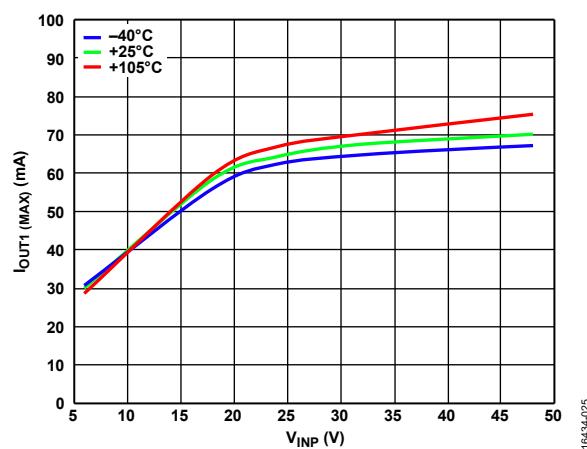
Figure 26. Flyback Regulator Maximum Output Current across Temperature, V_{OUT1} = 24\text{ V} , Using a Würth Elektronik 750316743 Transformer, Based on Target of 70% I_{LIM} (FLYBACK)
