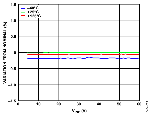
Figure 25. Flyback Regulator Line Regulation Across Temperature, V_{OUT1} = 21\text{ V} , I_{OUT1} = 20\text{ mA} , Nominal = V_{OUT1} with V_{INP} = 24\text{ V}
