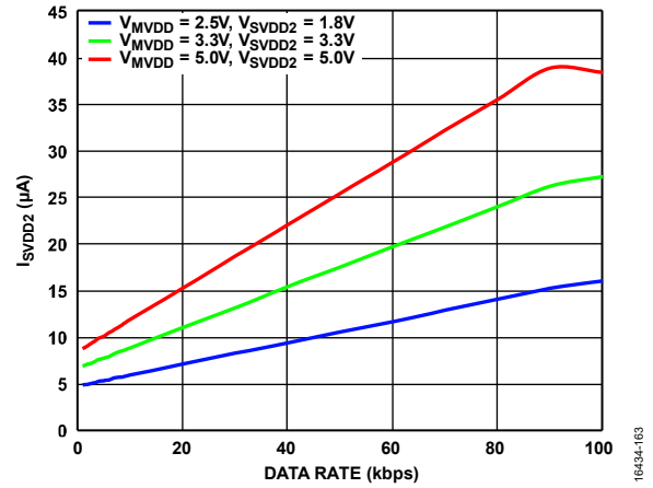
Figure 61. I_{SVDD2} vs. Data Rate on All GPIO Channels at Various Supply Voltages, \overline{MSS} Is High
