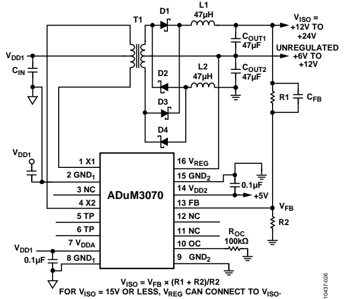
Figure 32. Doubling Power Supply
