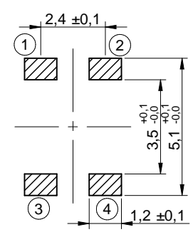
P.C.B Mounting Plan
