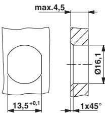
Dimensioned drawing
