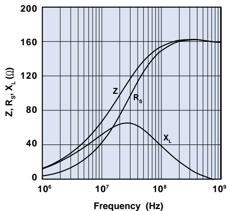
Figure 23A Impedance, reactance, and resistance vs. frequency for bead on lead 2743008112.
