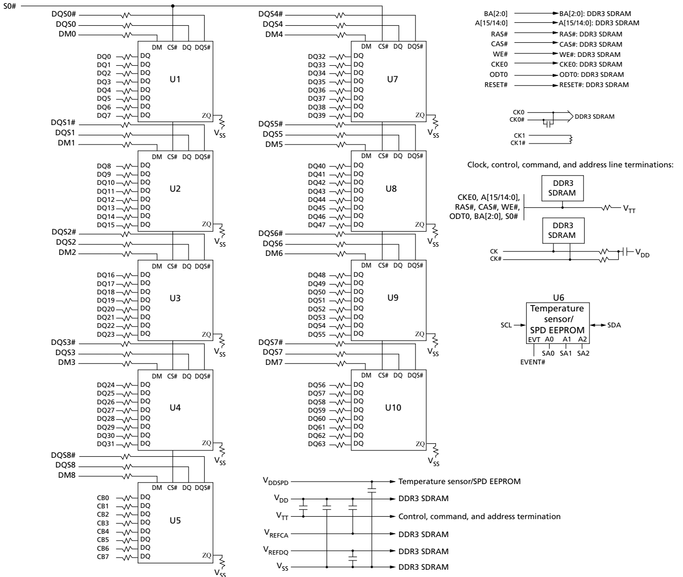
Figure 4: Functional Block Diagram (PCBs1483 & 1568)
