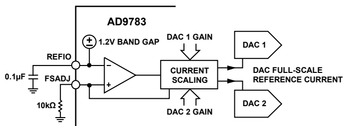
Figure 32. Reference Circuitry
