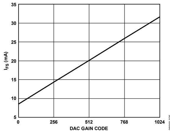
Figure 33. I_{FS} vs. DAC Gain Code
