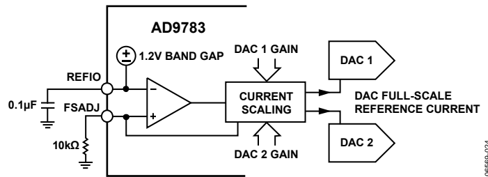
Figure 32. Reference Circuitry
