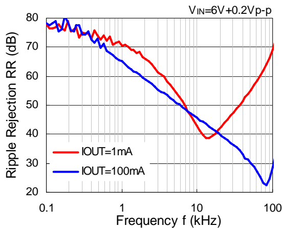
R1510S ( V_R=2.5\text{V} )
