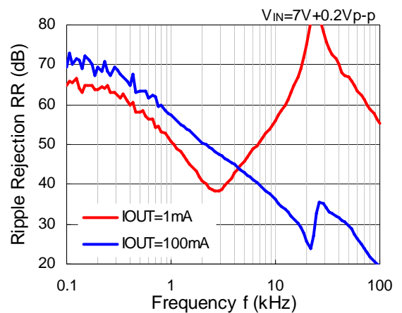
R1510S ( V_R=5.0\text{V} )
