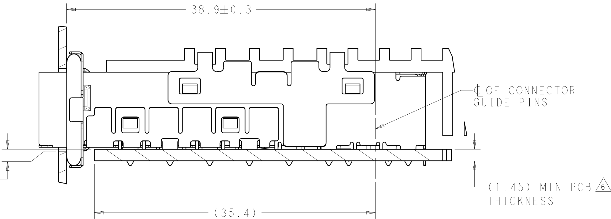
2170106-1 MOUNTED ON PCB SHOWN THRU RECOMMENDED BEZEL SCALE 4:1
