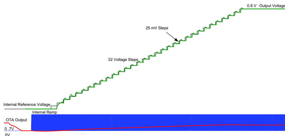
Figure 28. Soft-Start Details
