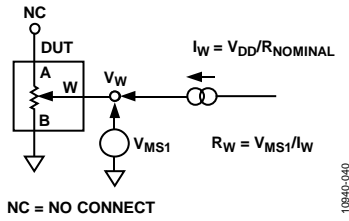
Figure 36. Wiper Resistance
