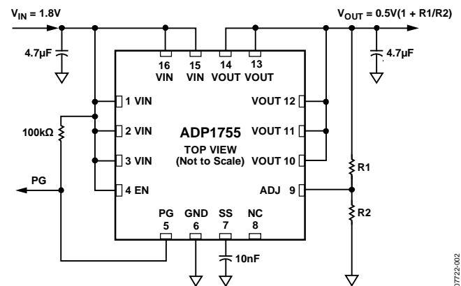
Figure 2. ADP1755 with Adjustable Output Voltage, 0.75 V to 3.3 V
