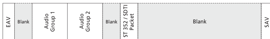
HANC with space between EAV and Ancillary Data (Audio Packets will be deleted)
