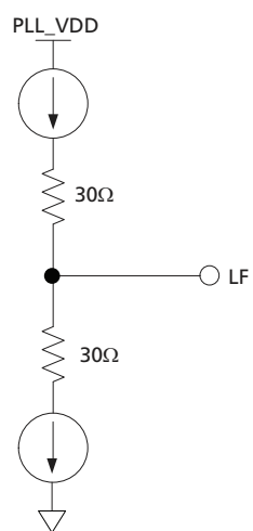
Figure 3-9: Loop Filter
