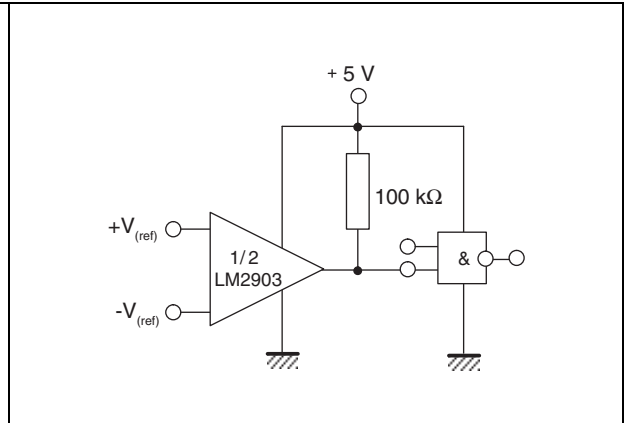
Figure 8. Driving CMOS
