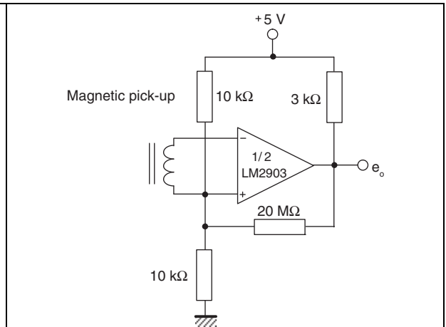
Figure 12. Transducer amplifier
