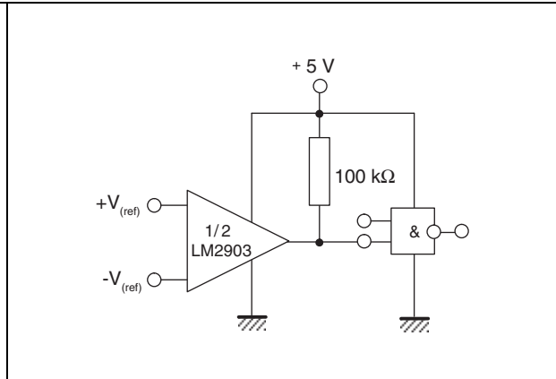
Figure 8. Driving CMOS
