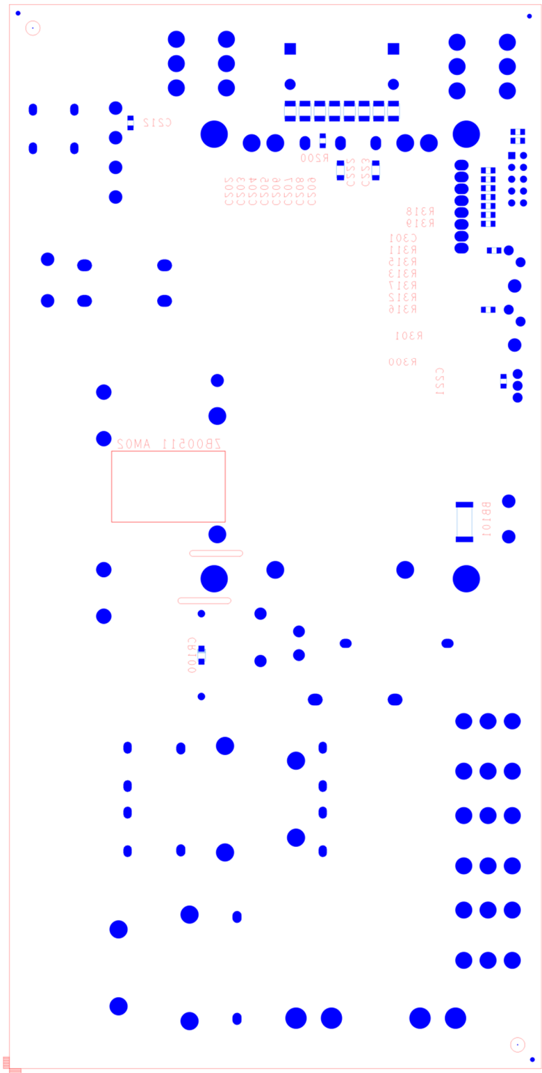
FIGURE 6 Bottom side Component Placement
