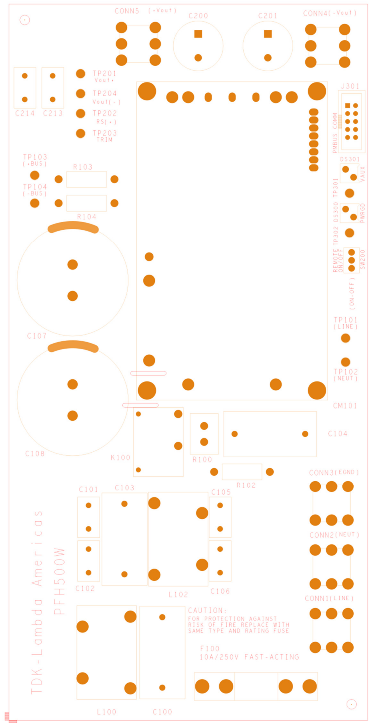
FIGURE 1 Top side Component Placement
