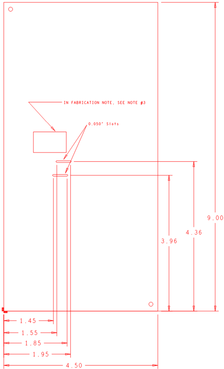
FIGURE 7 Circuit Outline
