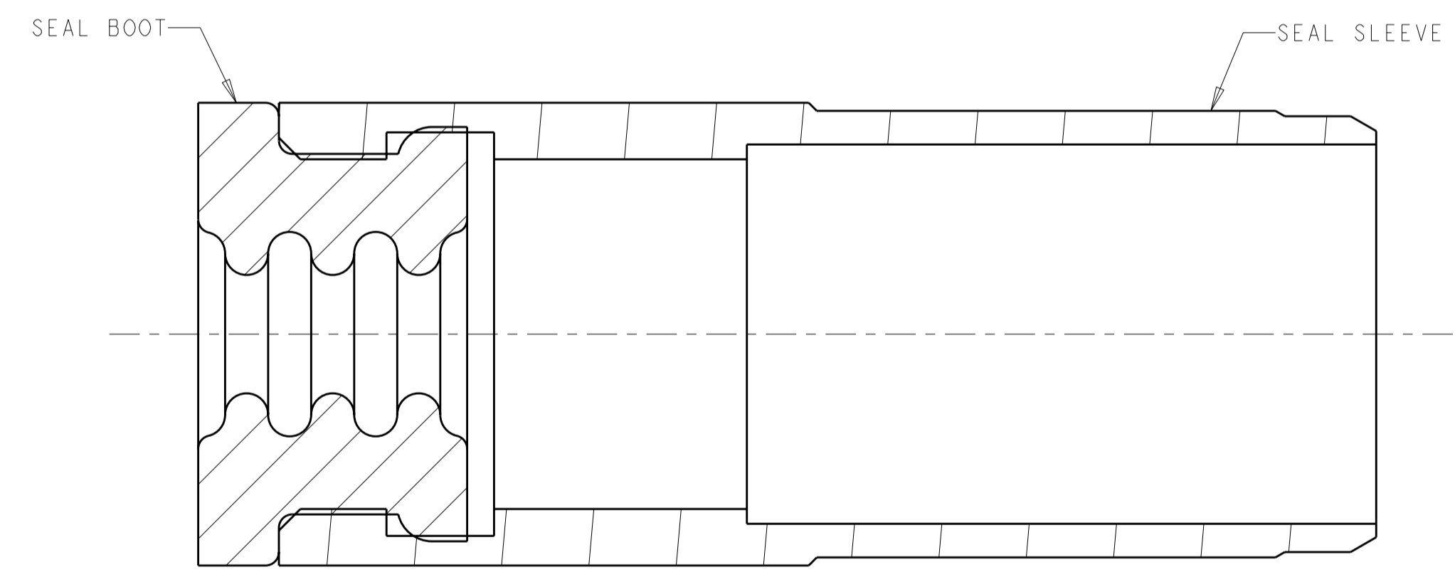
SECTION J-J
