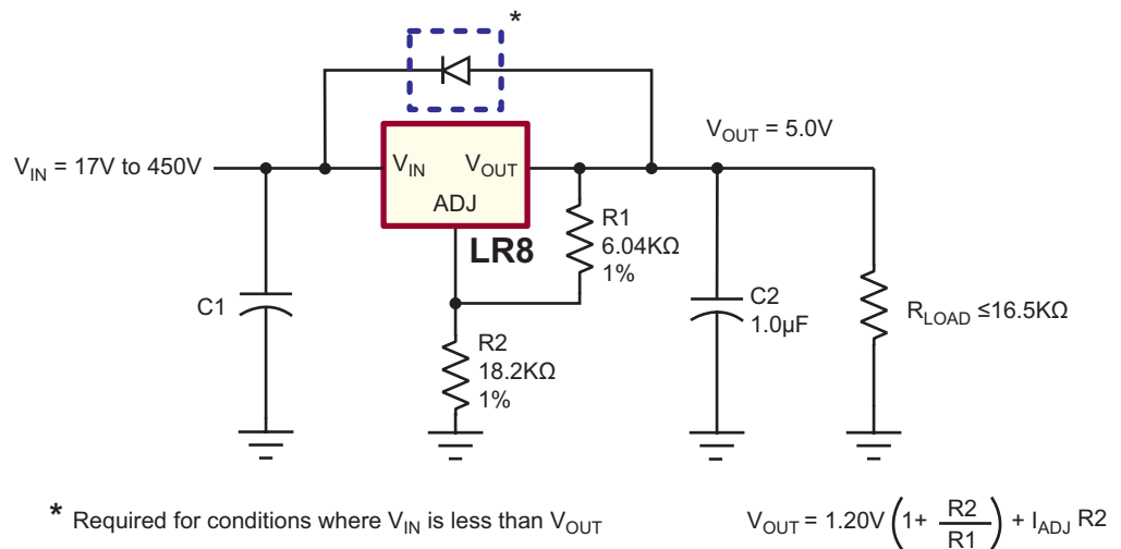
Figure 1: High Input Voltage, 5.0V Output Linear Regulator
