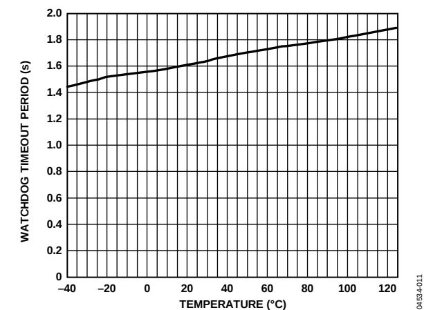
Figure 11. Watchdog Timeout Period vs. Temperature (ADM823/ADM824)
