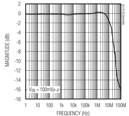
SMALL-SIGNAL RESPONSE
