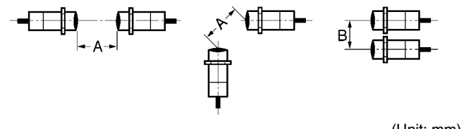
(Unit: mm)
