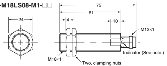
E2A-M18LS08-M1-□□
