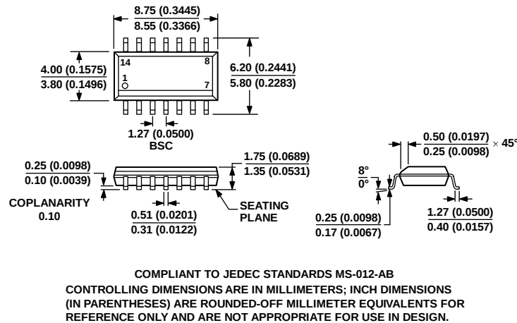
Figure 37. 14-Lead Standard Small Outline Package [SOIC_N] Narrow Body (R-14)
