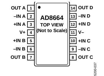
Figure 6. AD8664, 14-Lead TSSOP (RU-14)
