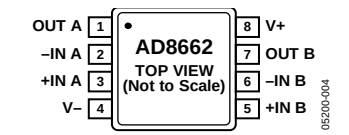
Figure 4. AD8662, 8-Lead MSOP (RM-8)
