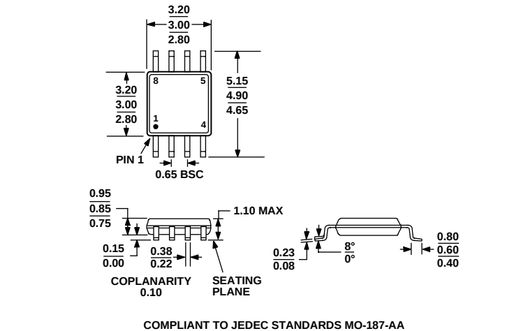
Figure 36. 8-Lead Mini Small Outline Package [MSOP] (RM-8)
