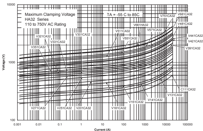
FIGURE 3. MAXIMUM CLAMPING VOLTAGE (V111HA32 - V751HA32)
