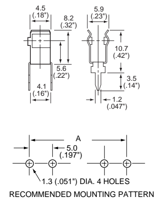
RECOMMENDED MOUNTING PATTERN
