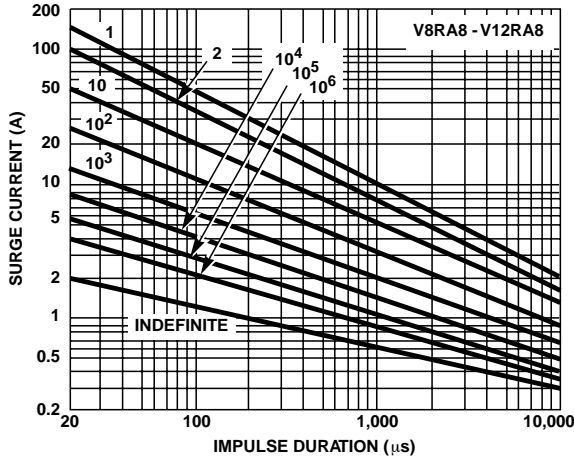
FIGURE 9. SURGE CURRENT RATING CURVES FOR V8RA8 - V12RA8
