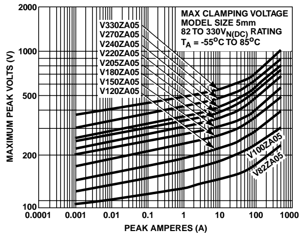
FIGURE 4. CLAMPING VOLTAGE FOR V82ZA05 - V330ZA05
