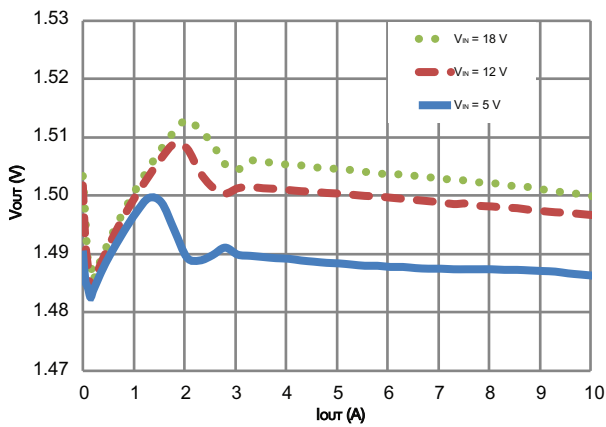
Figure 8 - Load Regulation - PSM (V DD = 5 V, V OUT = 1.5 V)
