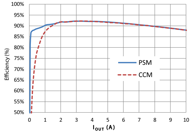
Figure 4 - Efficiency - PSM vs. CCM ( V_{DD} = 3.3\text{ V} , V_{OUT} = 1.5\text{ V} , V_{IN} = 12\text{ V} )
