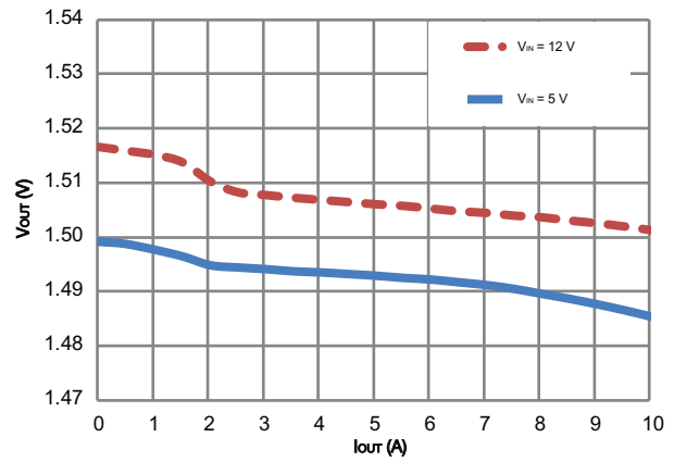
Figure 10 - Load Regulation - FCM (V DD = 3.3 V, V OUT = 1.5 V)
