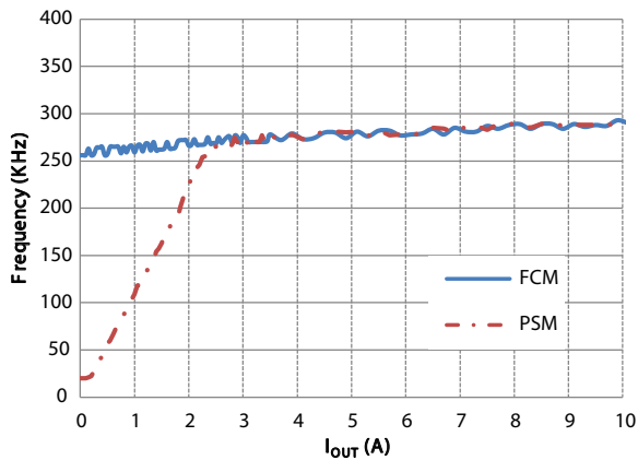
Figure 9 - Switching Frequency - PSM vs. FCM (V DD = 5 V, V OUT = 1.5 V, V IN = 12 V)
