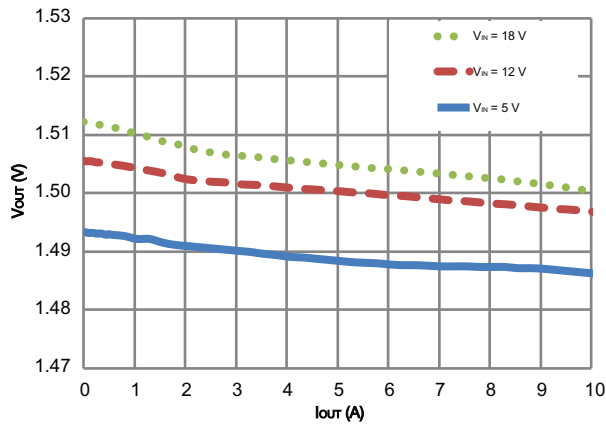
Figure 7 - Load Regulation - FCM (V DD = 5 V, V OUT = 1.5 V)
