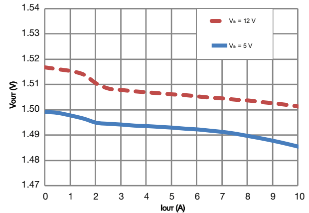
Figure 11 - Load Regulation - PSM (V DD = 3.3 V, V OUT = 1.5 V)
