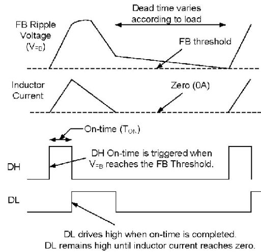
Figure 28 - Power-Save Mode
