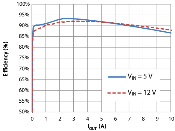
Figure 1 - PSM Efficiency - V_{IN} vs. Load ( V_{DD} = 3.3 V, V_{OUT} = 1.5 V)
