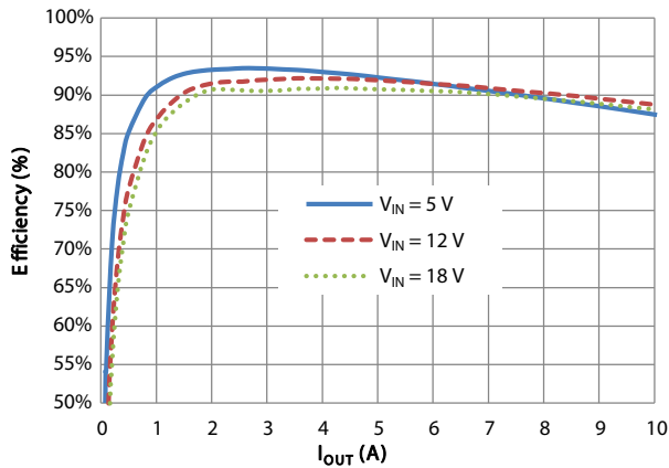
Figure 3 - PSM Efficiency - V_{IN} vs. Load ( V_{DD} = 5 V, V_{OUT} = 1.5 V)
