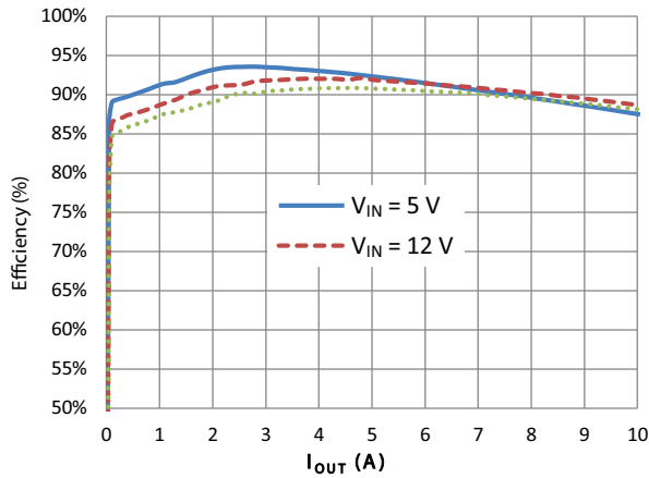
Figure 2 - PSM Efficiency - V_{IN} vs. Load ( V_{DD} = 5 V, V_{OUT} = 1.5 V)
