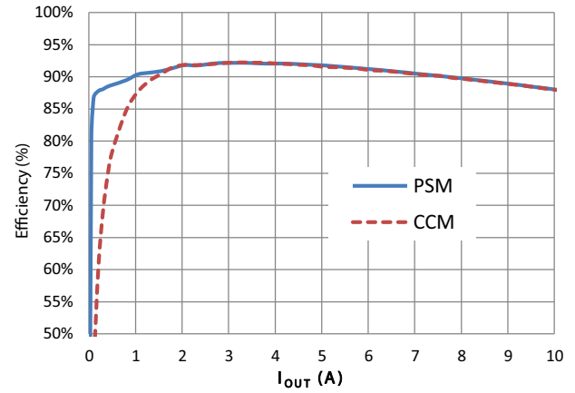
Figure 4 - Efficiency - PSM vs. CCM ( V_{DD} = 3.3 V, V_{OUT} = 1.5 V, V_{IN} = 12 V)
