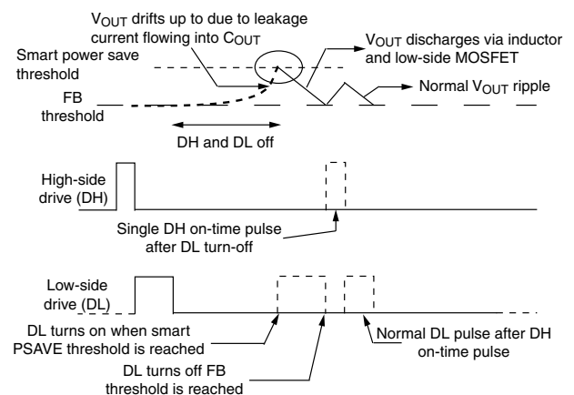
Figure 29 - Smart Power-Save
