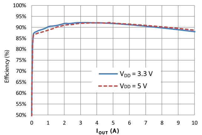
Figure 6 - PSM Efficiency - V_{DD} 3.3 V vs. 5 V ( V_{OUT} = 1.5 V, V_{IN} = 12 V)
