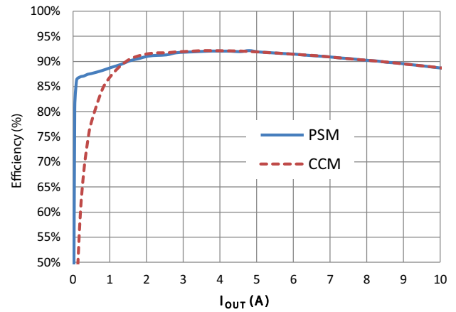
Figure 5 - Efficiency - PSM vs. CCM ( V_{DD} = 5 V, V_{OUT} = 1.5 V, V_{IN} = 12 V)
