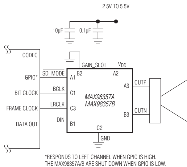
Figure 16. Left-Channel PCM Operation with 12dB Gain
