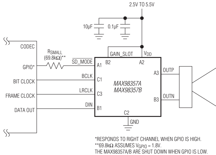
Figure 17. Right-Channel PCM Operation with 6dB Gain
