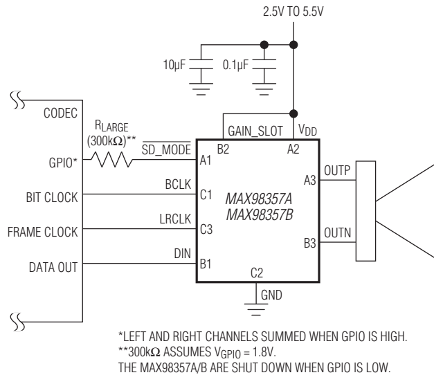
Figure 18. (Left/2 + Right/2) PCM Operation with 6dB Gain
