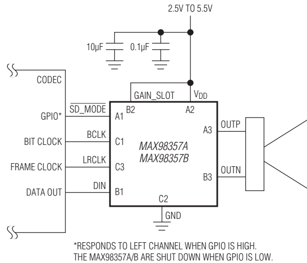
Figure 15. Left-Channel PCM Operation with 6dB Gain
