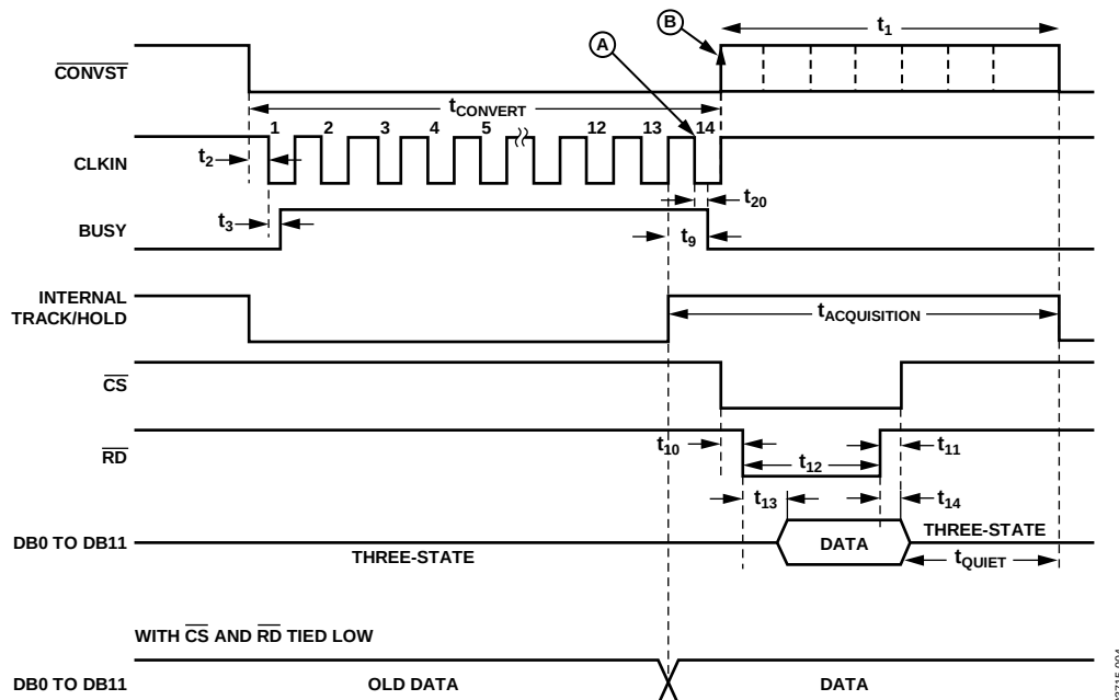
Figure 36. AD7938/AD7939 Parallel Interface—Conversion and Read Cycle Timing in Word Mode ( \text{W}/\overline{\text{B}} = 1 )
