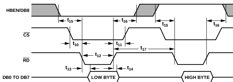
Figure 37. AD7938/AD7939 Parallel Interface—Read Cycle Timing for Byte Mode Operation ( \overline{W/\overline{B}} = 0 )
